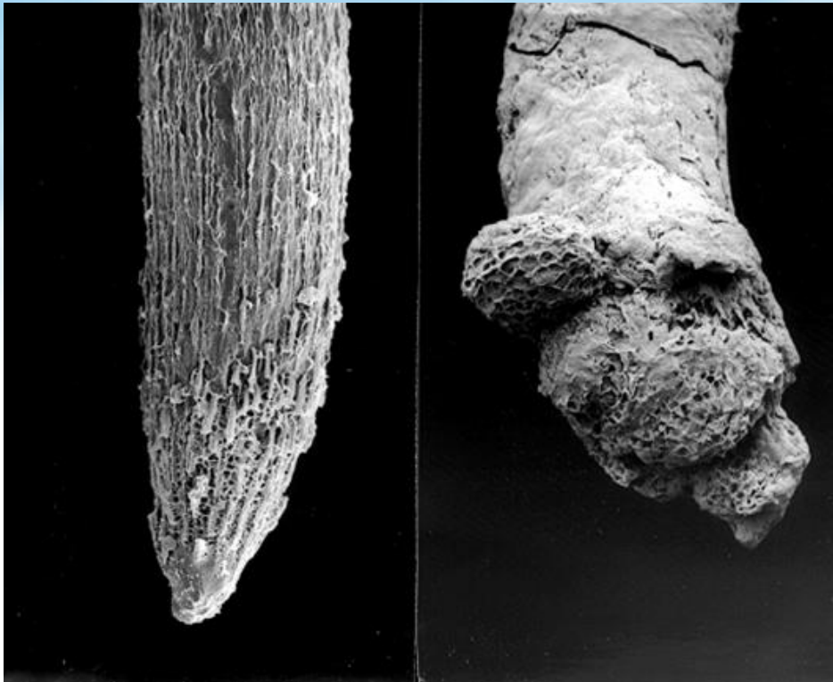
Wheat (Al 5 mg/kg, pH 5)
